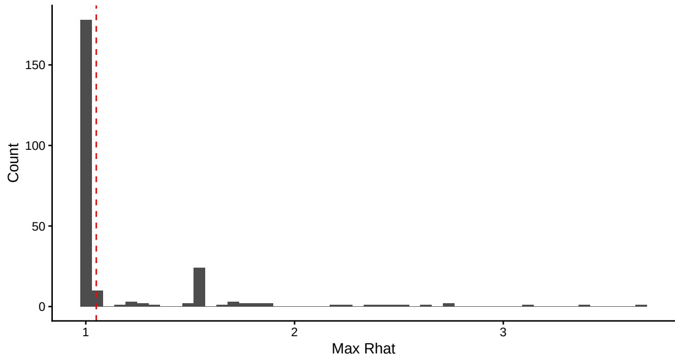
Maximum Rhat across recovery runs
